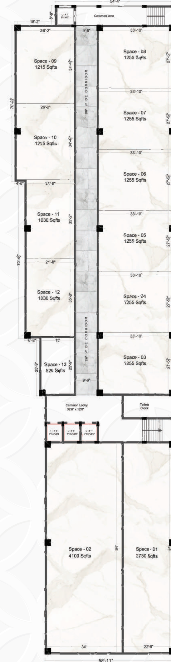
FIRST FLOOR
